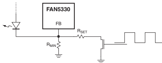
Figure 6. Dimming Using a PWM Logic Signal
